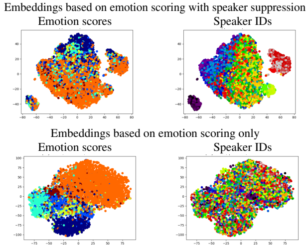
Figure 2: TSNE projection plots for differentially trained sequence to sequence embeddings (with overlapping speakers in the train and test datasets) on CREMA-D. The left side plots are colored with the emotion labels and the right side plots are colored with speaker IDs. The top pair of images are based on embeddings from the model trained on the loss function in equation 1 where w_{emo} > 0, w_{spk} > 0 . The bottom pair of images are based on a model where only emotion detection is trained.
