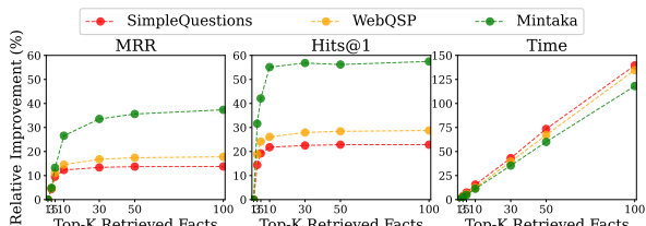
Figure 3: Performances and efficiencies of our DiFaR 2 with varying K , where we change the number of Top-K retrieved triplets when leveraging the reranking mechanism. We report results with the relative improvement (%) to our DiFaR without reranking. We report the time with average over 30 runs.
