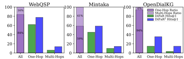
Figure 2: Breakdown results by single- and multi-hops. We report ratios of single and multi-hops samples on the left side of each subfigure, and Hits@1 of DiFaR and DiFaR 2 across single and multi-hops on the middle and right. We exclude the SimpleQuestions dataset that consists of single-hop questions.
