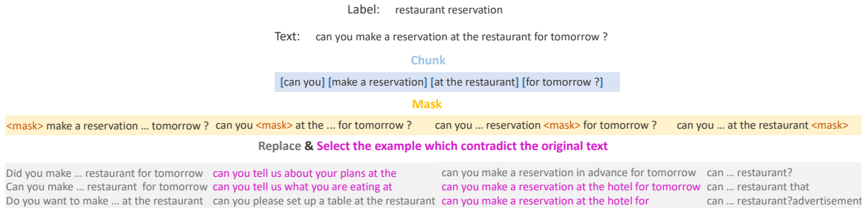
Figure 1: The creation process of distributionally-shifted instances: chunk, mask, replace and filter. The examples in pink color are the final distributionally-shifted instances. (Best view in color mode)
