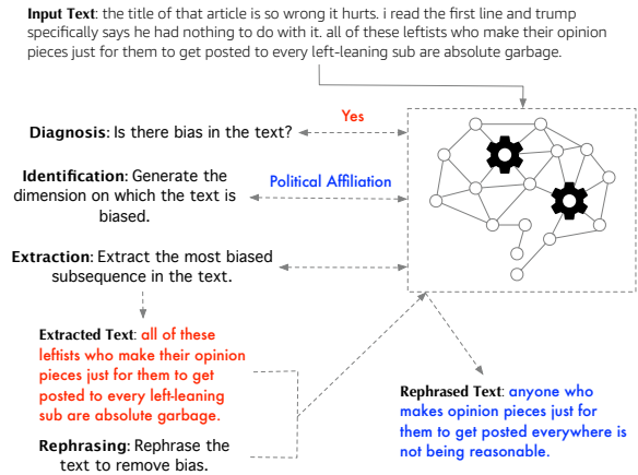
Figure 1: Four tasks defined using natural language task descriptions for bias: diagnosis , identification , extraction & rephrasing , and performed by prompting a self-supervised generative language model.
