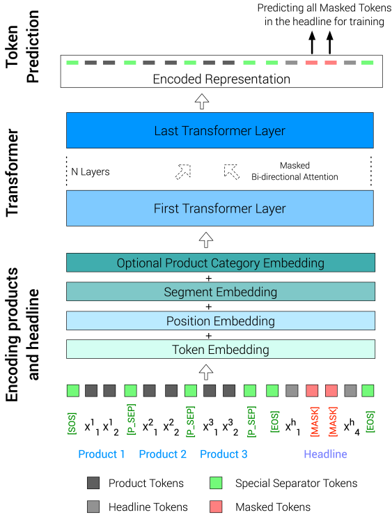
Figure 2: The sub-tokens from the product titles and headline are embedded and added with other embeddings that encode the positional and segment information. We also optionally add an embedding that represents the category of the product. During training, the masked tokens are predicted using Transformer layers and the cross-entropy (Eq. 2) loss and Self-Critical (Eq. 9) gradient is used to optimize the model. During inference, we predict one word at a time (left-to-right) in an auto-regressive manner using Beam Search.
