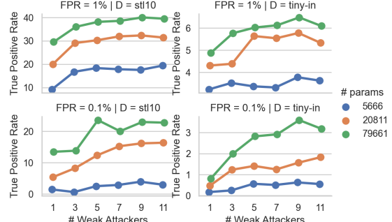
(b) Attacking Target Models with 32 Base Channels.
