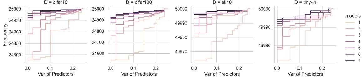
Figure 3: Variance Reduction of Bagging. We present CDF plots of variances of bagging predictors with an increasing number of quantile regression models on four datasets in our experiments. The x-axis indicates the variance estimated from 10 random runs, and the y-axis indicates the cumulative count of samples used in training the diffusion model. Ideally, with an increasing number of predictors in bagging, prediction variances of samples decrease, thus, more samples enjoy low prediction variances. We can see that, as the number of models increases in the bagging predictor, the CDF plot gradually becomes flatter, which means that the predictions on more samples now have lower variance. Thus, it shows that, by taking the majority vote of weak attackers, the prediction variance decreases, which results in better performance.
