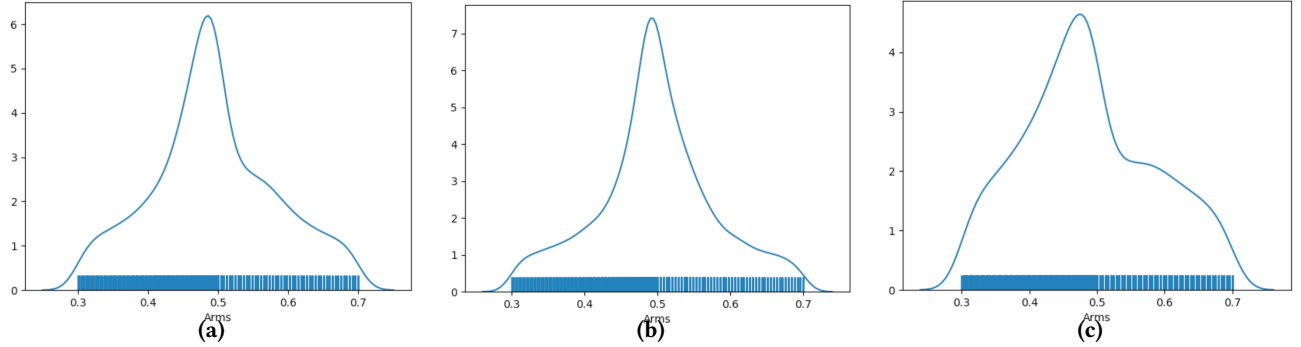
Figure 1: Kernel density estimate (KDE) of the distribution of arm pulls for real-valued arms in Experiment 2 (m=20) for three algorithms (a): MD-SAR , (b): MD-APT, (c): Proposed algorithm: MD-APT-ANY. MD-APT-ANY focuses its exploration budget on eliminating infeasible arms—note the peak of the distribution just less than the feasible boundary of 0.5.
