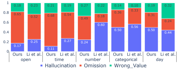
Figure 4: Error distribution across slot types
