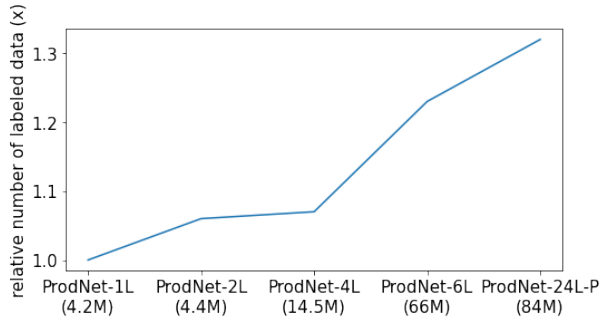
Figure 3: Relative number of labeled data required for active learning experiments to converge with model sizes on FEE dataset. e.g. , ProdNet-1L classifier requires x labels to converge while ProdNet-2L needs 1.06x labels to converge.
