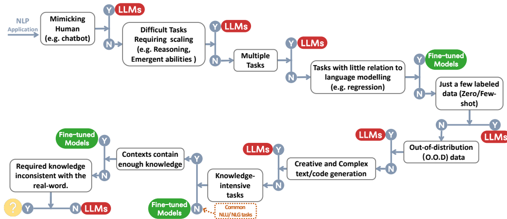
Fig. 2. The decision flow for choosing LLMs or fine-tuned models 21 for user’s NLP applications. The decision flow helps users assess whether their downstream NLP applications at hand meet specific conditions and, based on that evaluation, determine whether LLMs or fine-tuned models are the most suitable choice for their applications. During the decision process in the figure, Y means meeting the condition, and N means not meeting the condition. The yellow circle for Y of the last condition means there’s no model working well on this kind of application.
