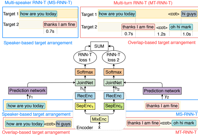
Fig. 1: Baseline MS-RNN-T with speaker-based target arrangement from [23], and proposed MT-RNN-T with overlap-based target arrangement with optional <cot> tag for speech segmentation. Model blocks with the same colour have tied parameters, transcripts in the colour-matched boxes belong to the same speaker.
