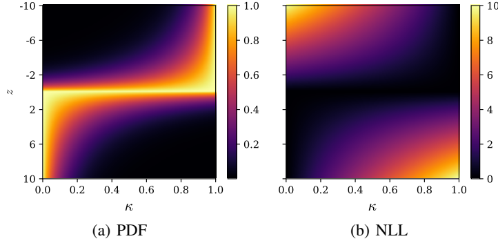
Figure 4: Probability density function (PDF) and negative log-likelihood (NLL) of the unnormalized Asymmetric Laplace Distribution for different quantile levels ( \kappa ) with m = 0 and b = 1 .
