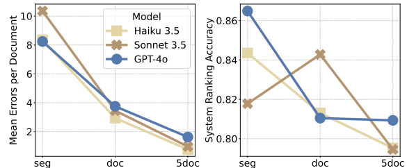
Figure 1: The number of predicted errors (left) and the average accuracy (right) for different input text granularities: segment-level, doc-level, and 5 doc-level.
