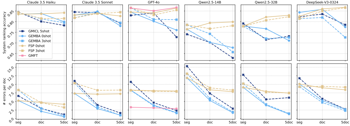
Figure 4: System ranking accuracy and number of error spans per document across methods and input granularities, averaged across translation directions. See Appendix B.4, B.5 for direction-specific results and character F1 scores.
