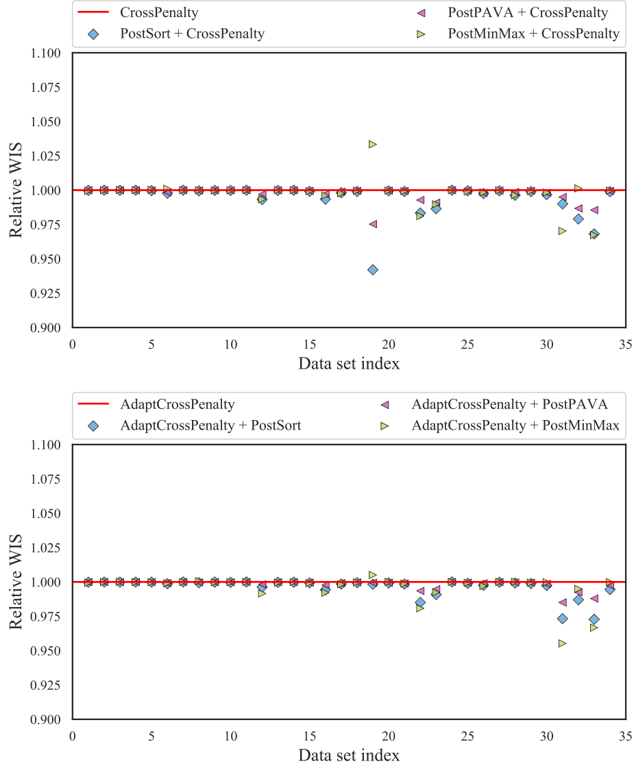
Figure 9: Comparing post isotonization strategies applied on top of CrossPenalty (shown in the top figure), and AdaptCrossPenalty (shown in the bottom figure). As we can see in either figure, PostSort and PostPAVA can only improve WIS; verifying Proposition 2. This is not true of PostMinMax, the most noticeable example being data set 19 in the top figure.
