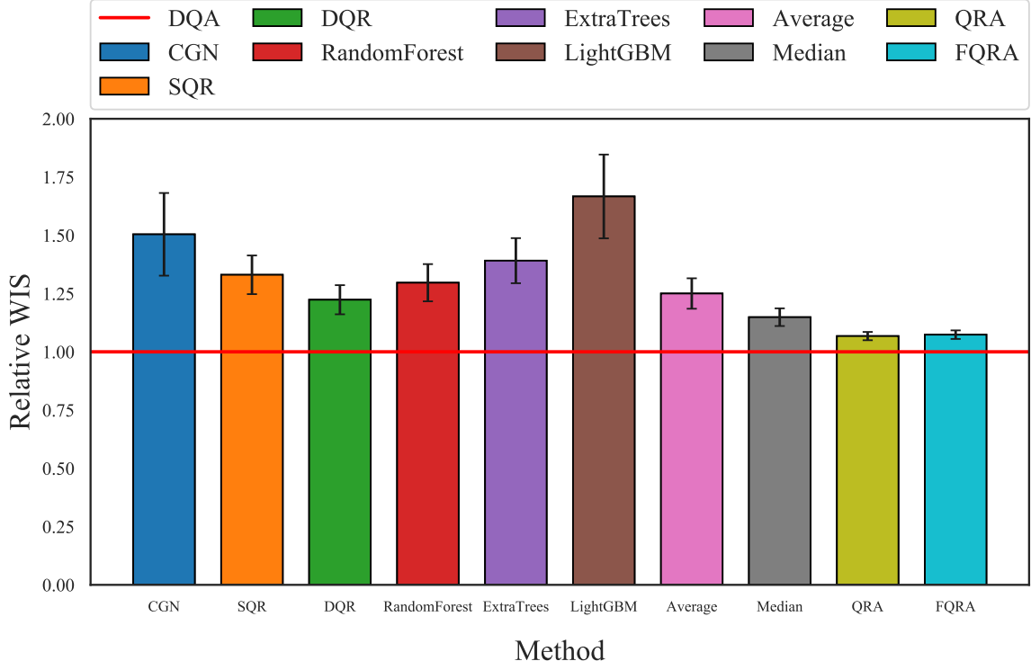
Figure 6: Average relative WIS over all data sets for deep quantile aggregation (DQA) and various quantile regression methods. The per-data-set results are given in Figure 1. Numbers larger than 1 indicate a worse average performance than DQA. We see that DQA performs the best overall, and QRA and FQRA are somewhat close runners up.
