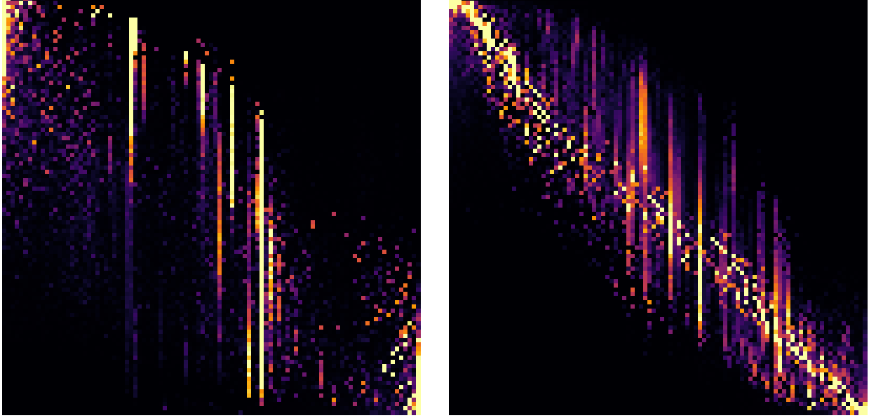
Figure 4: Heatmaps of aggregation weights fit by the local-fine (DQA) aggregator to the concrete data set (left) and the power data set (right). In the current fine setting, we have one m \times m = 99 \times 99 weight matrix per base model; the heatmaps have therefore been averaged over the p = 6 base models. Their rows correspond to the output quantiles (for the aggregator), and the columns to the input quantiles (from the base model). The right heatmap displays clear concentration around the diagonal: here each input quantile is on average the most reliable estimate used to define its corresponding output quantile. This is much less true on the left, which also has more pronounced vertical “streaks”: output quantiles use input quantiles from many neighboring quantile levels. The left heatmap also has notably more dispersion in the tails.
