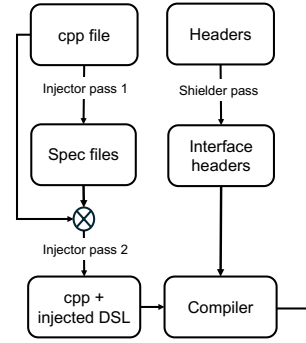
Figure 5: Build-time pipeline.
