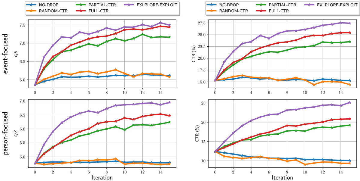
Figure 5: Average question scores and CTRs for the PARTIAL-CTR, CTR and EXPLPLOBE-EXPLOIT methods on general knowledge domain for personas with a single preference.
