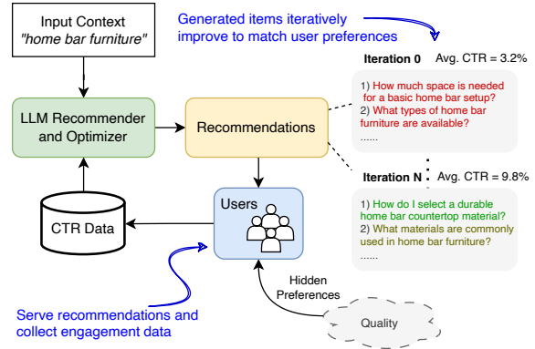
Figure 1: Overview of our generative recommender approach. It iteratively refines its item pool using feedback signals based on clicks to gradually improve the relevance of the questions to its user base.
