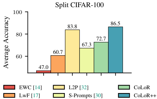
Figure 2: CoLoR improves by more than 5% on CIFAR-100 in the class-incremental scenario over S-Prompts.
