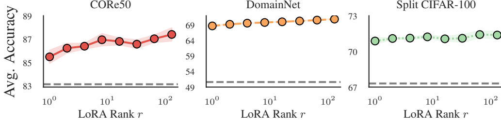
Figure 3: Increasing the rank by keeping all other settings fixed. Increasing the rank beyond 2-digit numbers yields only minor improvements in most cases. CoLoR outperforms its best competitor even with the smallest rank.
