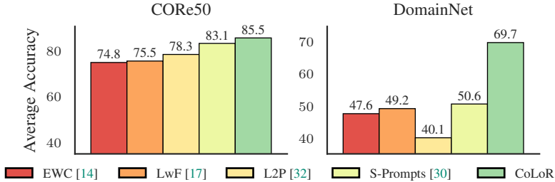
Figure 1: Results on two different datasets for domain-incremental learning. CoLoR improves by 2%-19% over the next best memory-free method.
