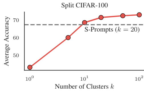
Figure 4: Increasing the number of clusters without changing any other setting. This significantly improves the performance in CIL (Split CIFAR-100) until k equals the number of new classes.
