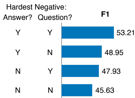
Figure 1: Ablation study for answer triggering. The columns on the left indicate whether online selection of hardest negative answer/question was done. To obtain best results with quadruplet loss, it is critical to sample both hard negative answers and hard negative questions.
