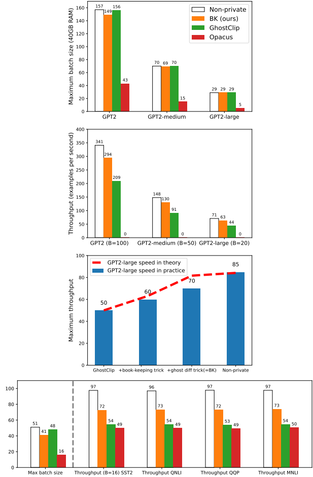
Figure 5. Memory and speed of different DP implementations. Upper: GPT2 on E2E dataset (fixing B , DP speed is 0.86 \sim 0.89 \times of non-DP). Lower: RoBERTa-large on GLUE datasets. Note here the hybrid implementations are equivalent to the base ones, because of the short sequence length.
