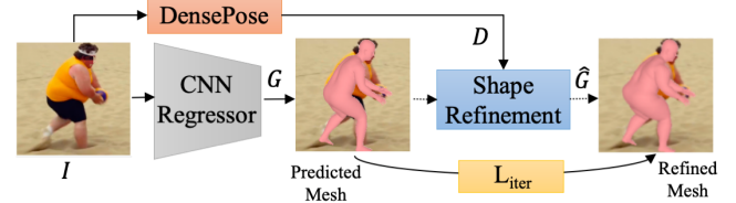
Figure 2. System Overview. Stage 1: A CNN Regressor is trained to estimate the SMPL parameters G using the L_{reg} loss (ref. Eq. (3)). Stage 2: The Shape Refinement module is initialized with G and runs an iterative optimization process with loss L_{iter} (ref. Eq. (4)) based on dense 3D correspondences D to produce updated parameters \hat{G} , used as pseudo-ground truth in the next epoch. Stage 3: At inference time, the trained regressor’s prediction G is refined using L_{iter} to produce the final fit.
