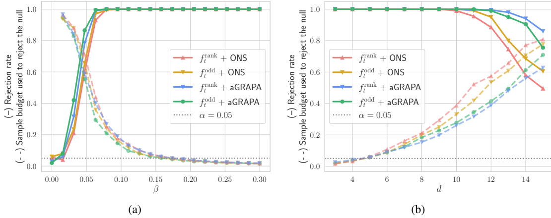
Figure 12. (a) Comparison of symmetry-based betting strategies under the Gaussian model. The betting strategy based on composition with an odd function performs only slightly better than the rank-based strategy. (b) SKIT with composition- and rank-based betting strategies under the spherical model. None of the betting strategies uniformly dominates the other. aGRAPA criterion for selecting betting fractions tends to result in a bit more powerful testing procedure.
