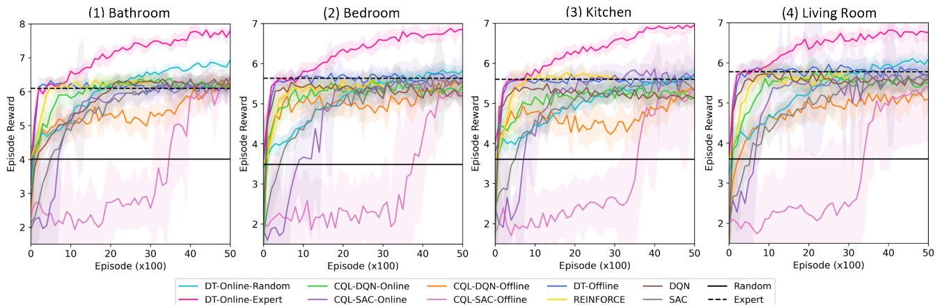
Fig. 4: Episode reward of proposed method and baselines in 4 categories of floor plans.
