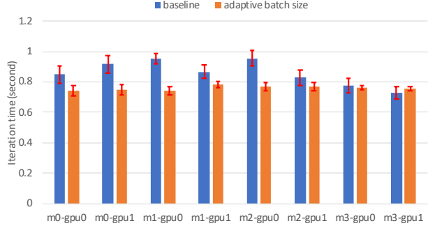
Figure 8. Iteration time (excluding backward and synchronization) of 8 trainers before and after batch size tuning
