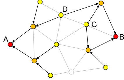
Figure 1. A mini-batch generated by a 2-layer neighbor sampling from two target nodes A and B. Orange nodes are the one-hop neighbors and yellow nodes are two-hop neighbors. Node C is shared by two neighbors of node B while Node D is covered by the receptive fields of both A and B.
