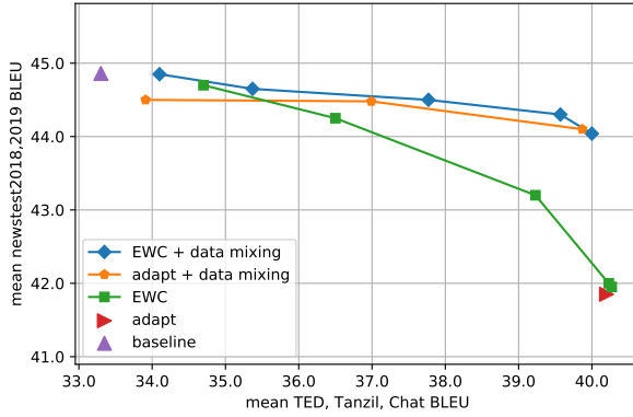
(a) DE→EN
