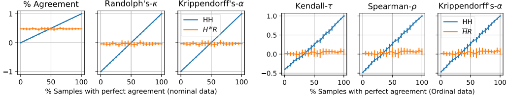
Figure 2: Simulating the impact of uncertainty by comparing with an automatic random labeler ( R ). When the proportion of samples with uncertainty is higher, even a random labeler can appear to have better correlation with a majority ( H^w ) or median ( \bar{H} ) human label. As the proportion of samples with consistency increases, the weakness of the random labeler become evident.
