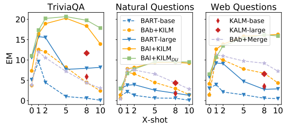
Figure 2: Results on QA datasets with different shots. BART results are in blue, while the results of BART+KILM are in orange and green. We use dashed and solid lines to denote the base- and large-size models, respectively. Also “BAB” and “BAI” correspond to BART-base and BART-large, respectively. KILM DU is KILM with data upscaling where entire Wikipedia articles are used instead of only their first paragraphs.
