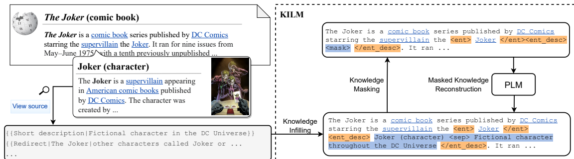
Figure 1: The illustration of the proposed KILM technique for injecting knowledge into PLMs. In the given example, the mention, Joker , is linked to the page of Wikipedia entity Joker (character) . While the figure only shows knowledge infilling, knowledge masking, and masked knowledge reconstruction steps, the proposed method is combined with the original pre-training objectives of PLMs for continued pre-training.
