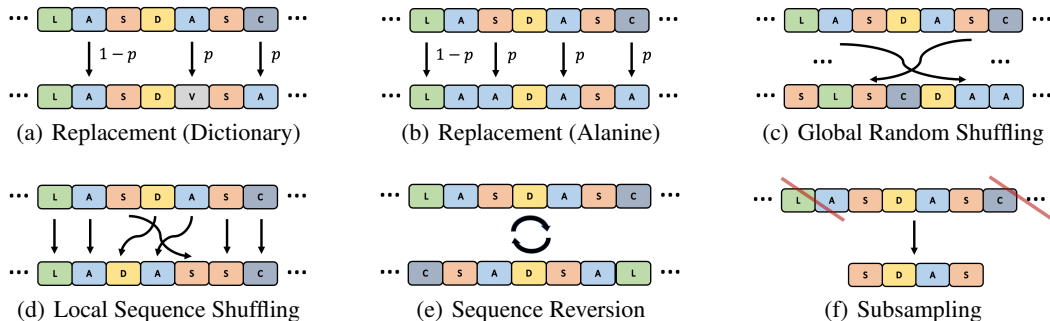
Figure 1: Diagram of data augmentations. We study randomly replacing residues (with probability p ) with (a) a chemically-motivated dictionary replacement or (b) the single amino acid alanine. We also consider randomly shuffling either (c) the entire sequence or (d) a local region only. Finally, we look at (e) reversing the whole sequence and (f) subsampling to a subset of the original.
