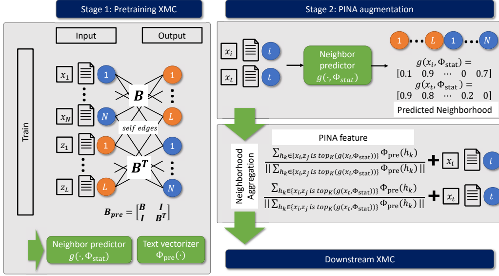
Figure 4. Illustration of the two-stage PINA method. At stage 1), we construct a pretraining biadjacency matrix B_{pre} using only the training data. Since we still have an XMC problem, we can train an XMC learner as the neighbor predictor g(\cdot, \Phi_{stat}) and obtain its corresponding text vectorizer \Phi_{pre}(\cdot) as well. At stage 2), we first use the pretrained neighbor predictor g(\cdot, \Phi_{stat}) to extract the most relevant (top K ) nodes among the output space of the pretraining task. Then we apply the pretrained text vectorizer \Phi_{pre}(\cdot) to obtain the numerical features for both instances and labels. Finally, we perform normalized neighborhood aggregation to obtain the PINA augmented features, which can then be used in downstream XMC.
