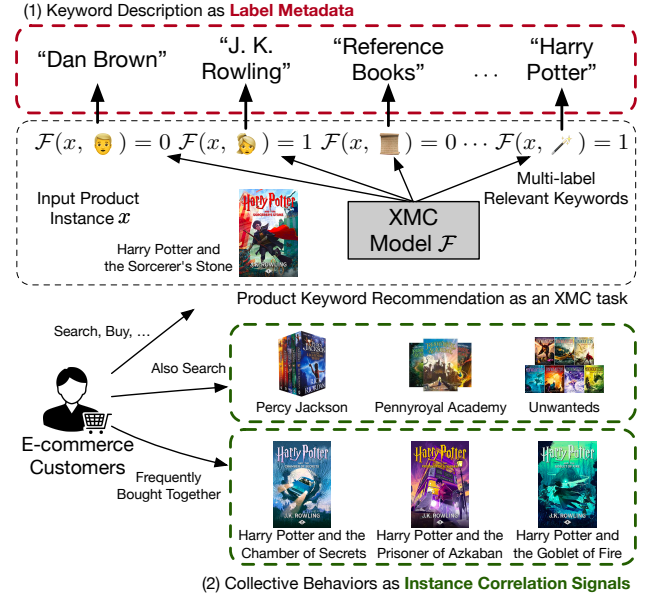
Figure 1. Illustration of two types of side information, including (1) label metadata and (2) instance correlation signals, based on an example XMC task that recommends relevant keywords (labels) for input products (instances) in E-commerce. Specifically, the text descriptions of keywords serve as label metadata while customer behaviors collectively provide instance correlation signals.
