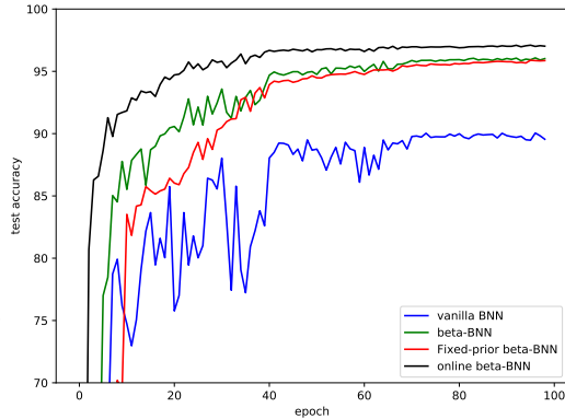
Figure 1: Testing accuracy over training epochs.
