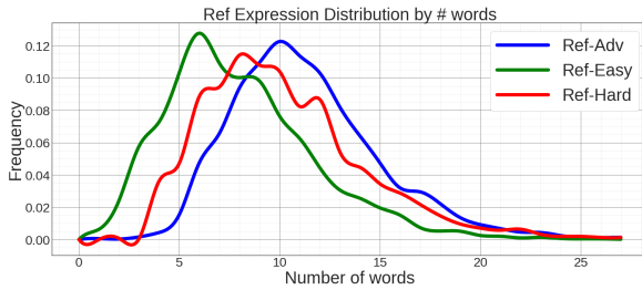
Figure 6: Referring expression length distribution for Ref-Easy , Ref-Hard , and Ref-Adv datasets.
