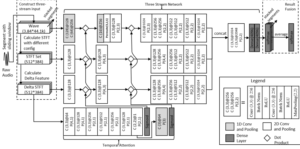
Fig. 1. System Architecture.
