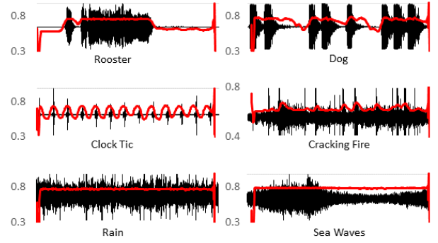
Fig. 2. Comparison of generated attention on environmental sound with different temporal structure. Black line: audio waveform, Red line: generated attention.
