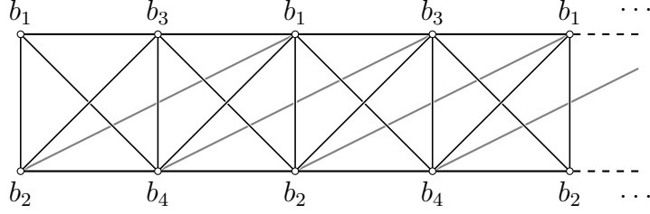
Fig. 4 Equipartition indifference graph for k = 4 , formed from the frustration graph of the Hamiltonian in Eq. (106). The Hamiltonian couplings are 4-periodic and are labeled b_1, b_2, b_3 , and b_4 .
