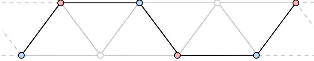
Fig. 1 The frustration graph of the model introduced in Ref. [4], which is (even-hole, claw)-free. Each of the sets of colored (red and blue) vertices are independent sets, and together they induce a path in the frustration graph. In a general claw-free graph, the symmetric difference of any pair of independent sets induces a bipartite subgraph of maximum degree two: all of the components of the subgraph are induced paths and even-holes. If the graph is furthermore even-hole free, then the symmetric difference induces a set of disjoint paths.
