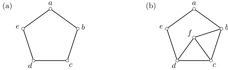
Fig. 2 Frustration graphs for small system sizes solved in this section: (a) a five-cycle, which admits a generator-to-generator mapping, but is both even hole and claw free also, thus admitting a solution by the method developed in the present work, (b) one of the six forbidden subgraphs of a line graph with no twins, created by adding a single additional Hamiltonian term to the five-cycle, thus when f \rightarrow 0 , this model is identical to (a). This model does not admit a generator-to-generator mapping, but is solvable using the method developed here.
