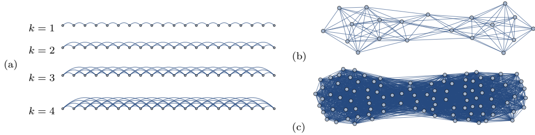
Fig. 3 Indifference frustration graphs for some simplicial ECF models (see text). (a) Equipartition indifference graphs arise, for example, as frustration graphs for the translation-invariant spin chain (having open boundary conditions) with Hamiltonian H_k = \sum_i X_i X_{i+1} \cdots X_{i+k-1} Z_{i+k} . The frustration graph is shown for k = 1, \dots, 4 . When k = 1 , a Hadamard rotation on every second spin shows that this model is equivalent to the XY model with half of its terms removed, and it can be solved by a Jordan-Wigner transformation. The k = 2 model is the model studied by Fendley [4]. When k \geq 2 , the graph is not a line graph, so it cannot be solved by any Jordan-Wigner transformation [3], but since it is simplicial and ECF by construction, it can be solved by the methods introduced in this paper. (b,c) Two examples of simplicial ECF graphs that arise as indifference graphs with randomly chosen points at different densities. It is evident that, depending on the point density, the connectivity of interval graphs can look rather complex.
