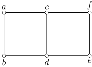
Fig. 7 The frustration graph of the model, defined in Equation (120). This model has claws and even holes, nevertheless for all-equal-coefficients the model has a free fermion spectrum.
