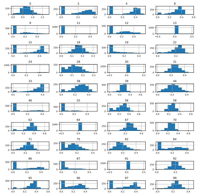
Figure 9: Objectives selection for Yahoo! Learning to Rank dataset. We plot the histogram of the standard deviation of the feature per query group. We then select the features that have the most diversified values per query group.
