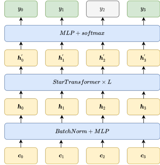
Figure 1: Model architecture. We take the columns c_0, c_1, c_2, \dots as inputs, and apply batch normalisation to multi-layer perceptron (MLP), which is followed by L layers of Star Transformer. We then use a MLP with softmax function to classify over a set of target concept types. Columns with missing labels are ignored (here y_2 ).
