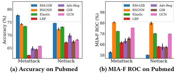
Figure 3: Results on perturbed Cora and Pubmed graphs.
