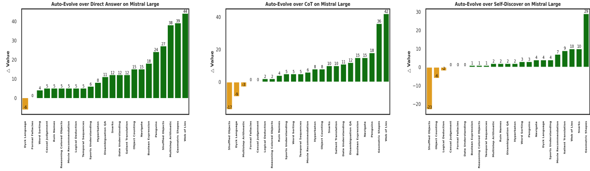
Figure 4: Task level BBH performance on Mistral Large for Auto-Evolve over Direct Prompt, CoT and Self-Discover. Claude models and GPT-4 results are in Appendix Fig. 12 and Fig. 13
