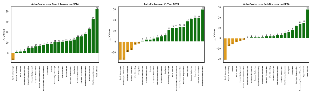
Figure 12: Performance comparison between Auto-Evolve and Direct Prompt, CoT and Self-Discover on GPT-4.
