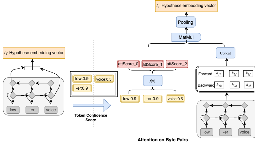
Figure 6: Attention on byte pair embedding.
