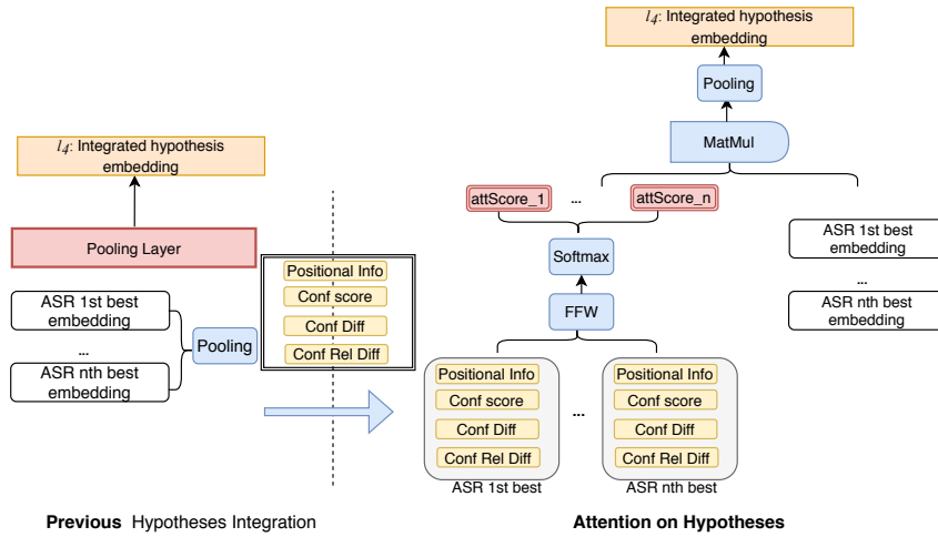
Figure 7: Attention on hypotheses integration.
