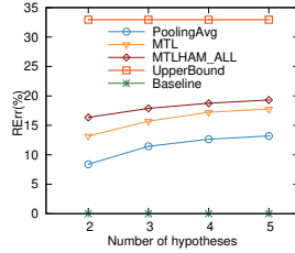
Figure 9: Comparison under different amount of n -bests.
