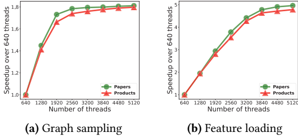
Figure 2. Execution speed for the graph sampling and feature loading kernels of Quiver when changing physical threads. One GPU with 5120 physical threads is used.
