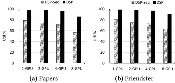
Figure 6. GPU utilization for sequential execution (DSP-Seq) and the pipeline, experiment settings detailed in Section 7
