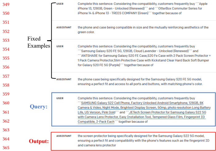
Figure 3: Explanation on Cellphones generated by ChatGPT.
