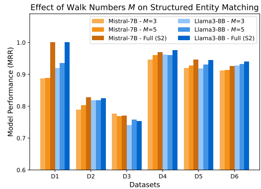
Figure 3: Effect of Walk Numbers M on LLMs with Fine-tuning for Matching Tabular and Semi-structured Entities. M represents the number of entity attributes sampled in the serialized input, and increasing M eventually leads to the input sequence equivalent to S2 Random order without downsampling.
