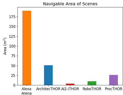
Figure 6: Bar plot of the navigable areas for Alexa Arena, comparing to ArchitecTHOR, AI2-iTHOR, RoboTHOR and ProcTHOR.
