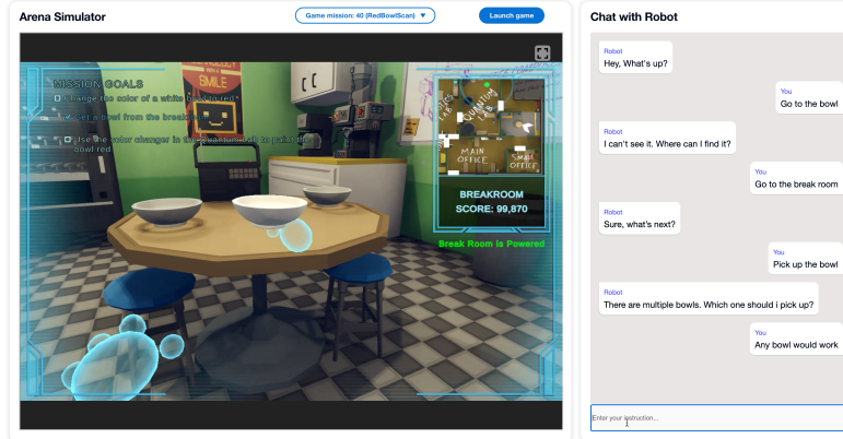
Figure 2: The web-based user interface. The user can use the chat box to communicate with the agent in Arena for task completion. Meanwhile, video from Arena is streamed in real time to show the progress. The minimap is displayed on the top right corner of the game UI, showing the room layout and the robot location and orientation. The mission goal and subgoals are displayed to the users in text on the top left corner of the UI.
