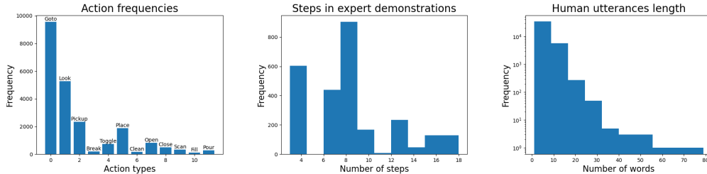
(a) Frequencies of action types. (b) Steps in expert demonstrations. (c) Length of human utterances.
