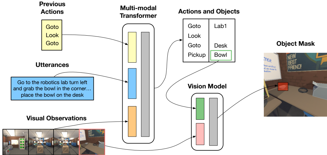
Figure 13: Model architecture for the Neural-Symbolic approach which uses unshared modules to predict actions and masks, and heuristic rules for visual grounding.
