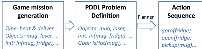
Figure 8: Process of generating game missions and expert demonstrations.
