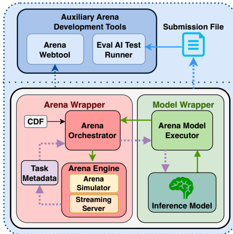
Figure 5: Overview of Alexa Arena Platform Architecture. The core modules are the arena wrapper and model wrapper . The arena engine contains the simulator and the streaming server . The metadata from the Arena Engine are sent to the inference model, which generates actions to be executed in the simulator. We have also built infrastructure to generate results submission files for EvalAI challenges.
