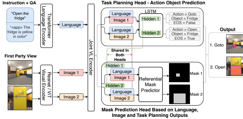
Figure 4: Model architecture of the vision language model for end-to-end action prediction and visual grounding.
