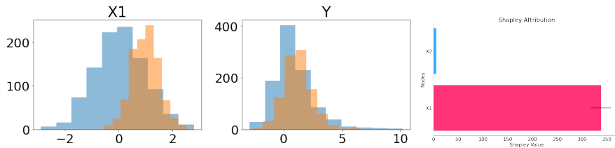
Figure 4: Data distributions for x_1 (left) and output y (middle) for two datasets, represented in blue and orange respectively. Shapley value attributing the changes of outputs to changes in inputs (right).
