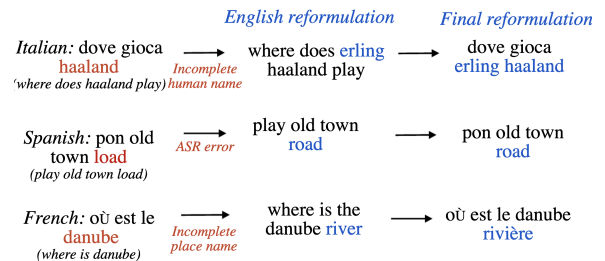
Figure 1: Examples demonstrating how CL-QR works. The defective non-English queries are first mapped to English to get the English reformulations, and then transferred to final reformulations in the original language.
