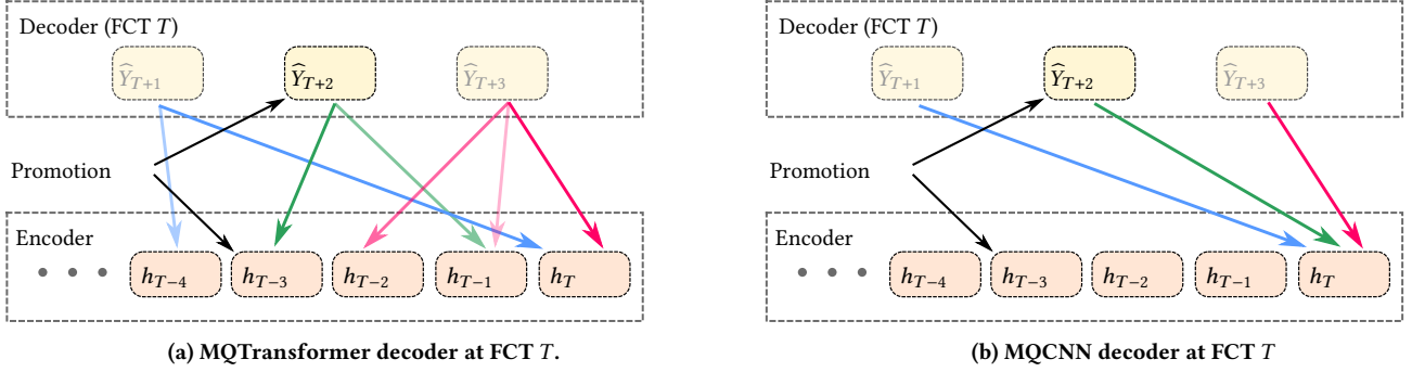
Figure 1: Example of a demand forecasting task where periods T-3 and T+2 both have promotions. The encoded context h_{T-3} , the last time the item had a promotion, contains useful information for forecasting for target periods that also have a promotion. The horizon-specific attention aligns past encoded contexts with the target horizon.
