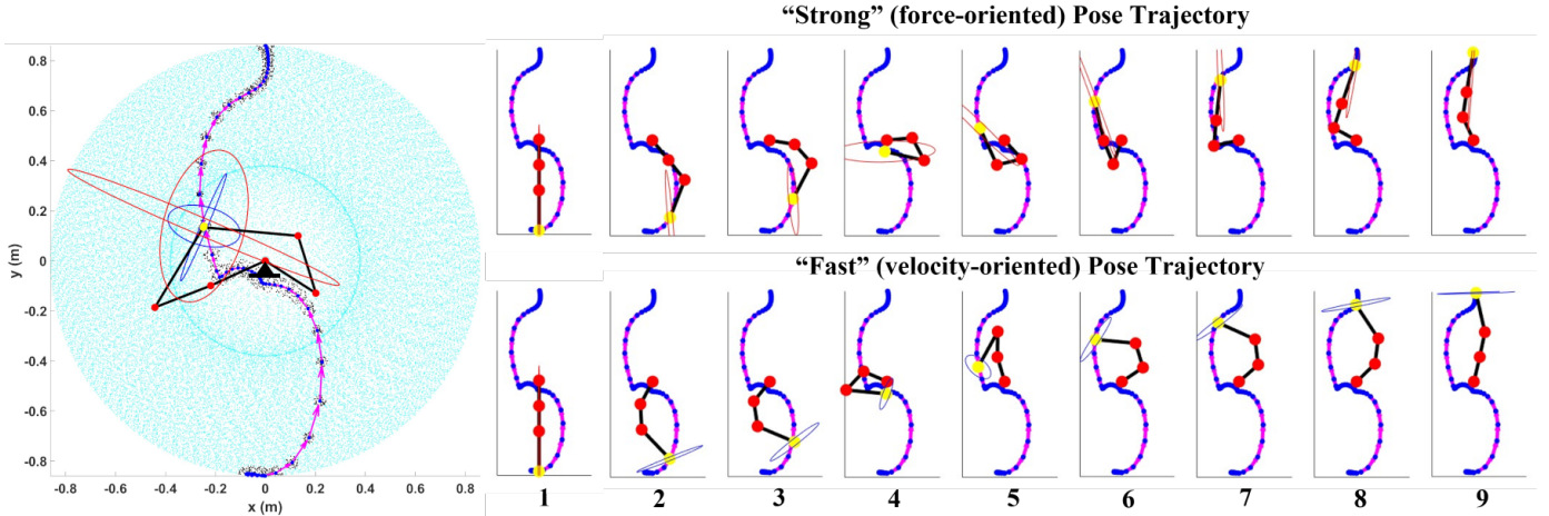
Fig. 2: Kinematic planning based on velocity and force ellipses. (Left) 2D Workspace of the manipulator was sampled (cyan points) and a discrete predefined trajectory was defined (blue dots) with nearest neighbors (black) and motion direction (magenta) marked at each trajectory waypoint. As an example, two pose candidates were generated at a certain waypoint with their velocity (blue) and force (red) ellipses. (Right) The motion sequence of “strong” and “fast” pose trajectories with corresponding ellipses.
