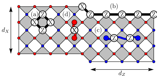
FIG. 9. Initialising a hexon surface code. Red(blue) vertices are initialised in Pauli-X(Pauli-Z) basis. The system is prepared in an eigenstate of shaded plaquettes (a) and the logical Pauli-Z operators, (b). This initialisation strategy is robust to biased noise. Pauli-Z errors that can occur on red vertices are detected by the shaded plaquettes (c). We can also detect low-rate Pauli-X errors on blue vertices with using this method of initialisation, see (d).
