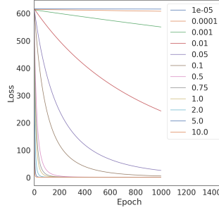
Figure 2: Loss histories corresponding to fixed LRs for NMF with SGD.
