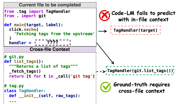
Figure 1: CodeGen-2B-mono fails to complete a Python program correctly as in-file context does not provide sufficient information. The model needs to know that TagHandler takes an argument raw_tags , which could be obtained through the function list_tags of git . Generating the correct code requires the presence of class and function definitions as part of the context, which cannot be derived from the current file alone.
