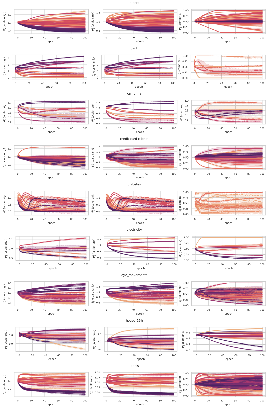
Figure 8: Weights learned by the proposed approach on all 14 datasets, part 1.
