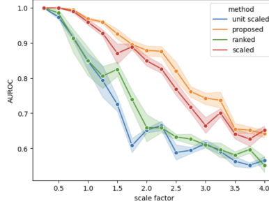
Figure 4: AUROCs of MLPs using the baseline transforms and the proposed method over multiple scale factors. As the scale factor increases, the target function frequency of the dataset also increases. Shaded regions correspond to 95% confidence intervals across 10 random seeds.
