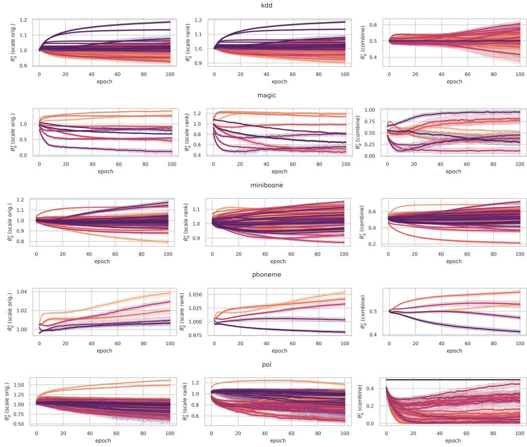
Figure 9: Weights learned by the proposed approach on all 14 datasets, part 2.
