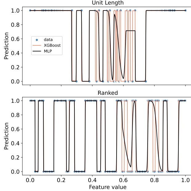
Figure 7: (Top) Data with labels varying over small distances are difficult for neural networks to learn, but easy for tree-based methods. (Bottom) Transformations that redistribute the data can increase the scales over which the feature labels vary, effectively lowering the frequency of the target function and making it easier for a neural network to learn.
