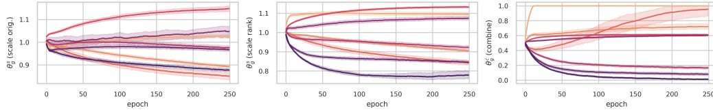
Figure 3: Weights learned by the proposed approach on electricity dataset. Lines represent values taken by the weights \theta_g throughout 250 epochs, and shaded regions represent the 95% confidence intervals. The weights consistently converge to similar values across 10 random seeds that vary data splits and neural network initializations. Due to heterogeneous nature of tabular datasets, scaling and ranking weights that minimize the loss for different features are different.
