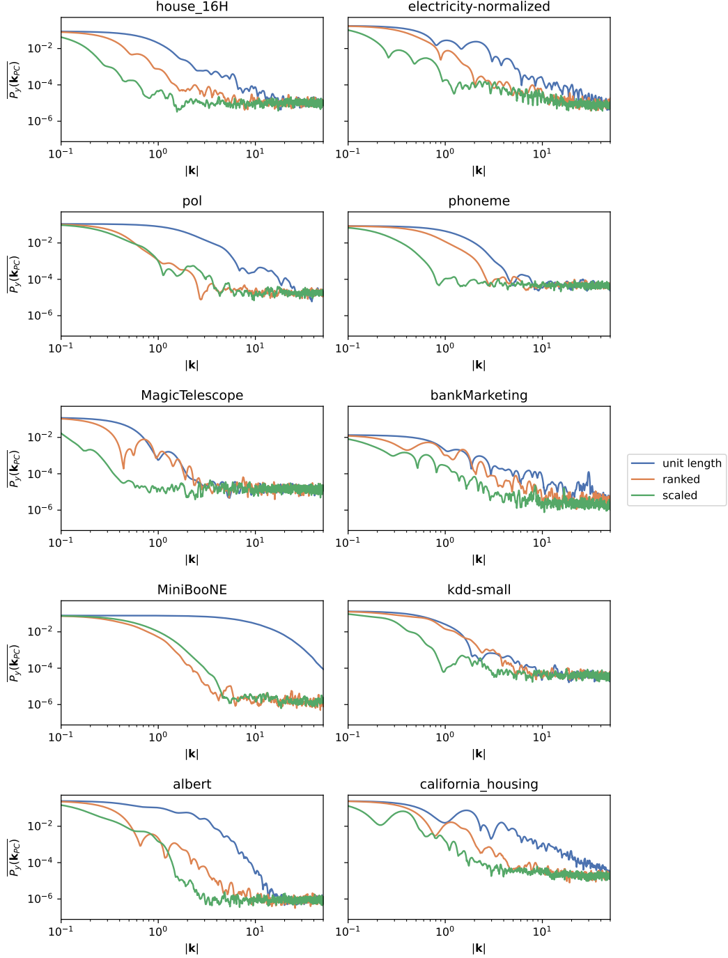
Figure 5: Spectra for binary classification training datasets determined by Equation (1) for the rank and scale transformations, compared to the datasets with unit length features. Results are marginalized over 10 different random seeds for the train-test split, and over \mathbf{k}_{PC} corresponding to the 1st PC after each transformation is applied. The solid lines are the resulting mean values, with shaded regions representing the 95% confidence intervals. Different transformations significantly affect target function frequency spectra.
