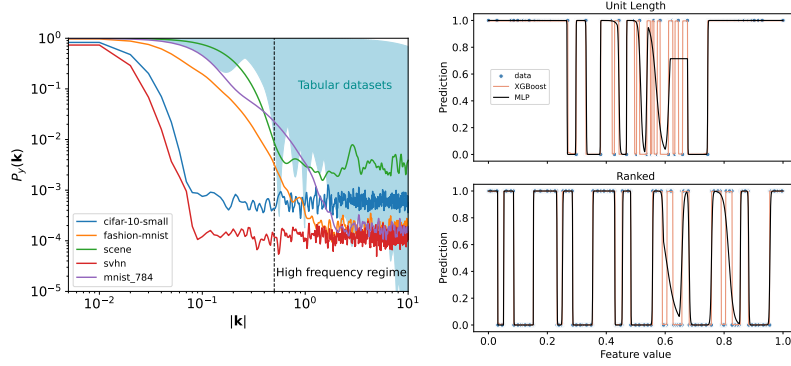
Figure 1: (Left) Due to their heterogeneous nature, tabular datasets tend to describe higher frequency target functions compared to images. The spectra corresponding to image datasets (curves in color) tend to feature lower Fourier amplitudes at higher frequencies than heterogeneous tabular datasets (cyan region). (Top Right) Data with labels varying over small distances are difficult for neural networks to learn, but easy for tree-based methods. (Bottom Right) Ranking is a transformation that redistributes the data and increases the scales over which the feature labels vary. This transformation effectively lowers the frequency of the target function, making it easier for a neural network to learn.
