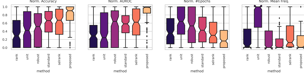
Figure 2: Normalized measurements of performance, convergence and frequency across datasets and seeds. The simple frequency-informed approach, selrank, with rank implemented as quantile transform improves upon rank alone. Additionally, our proposed methods significantly outperform all baselines, while converging faster.
