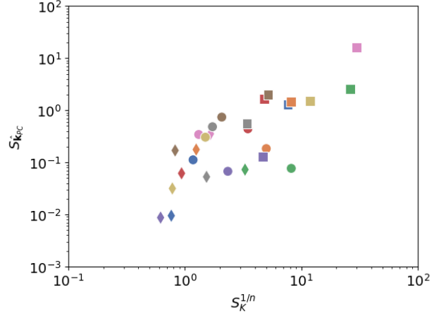
Figure 6: Comparison of different methods for quantifying the spectral energy at high frequencies. The horizontal axis corresponds to Equation (21), and the vertical axis to Equation (2). Squares, circles, and diamonds correspond to unit-scaled, rank, and scale features, and the different colors correspond to different datasets. The two methods are highly correlated.
