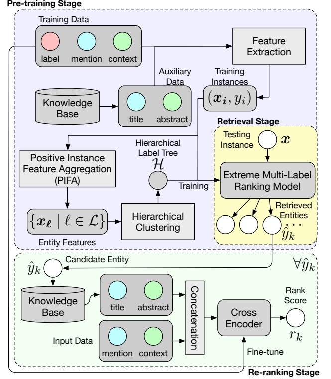
Figure 1: The overall illustration of the XMRED framework.
